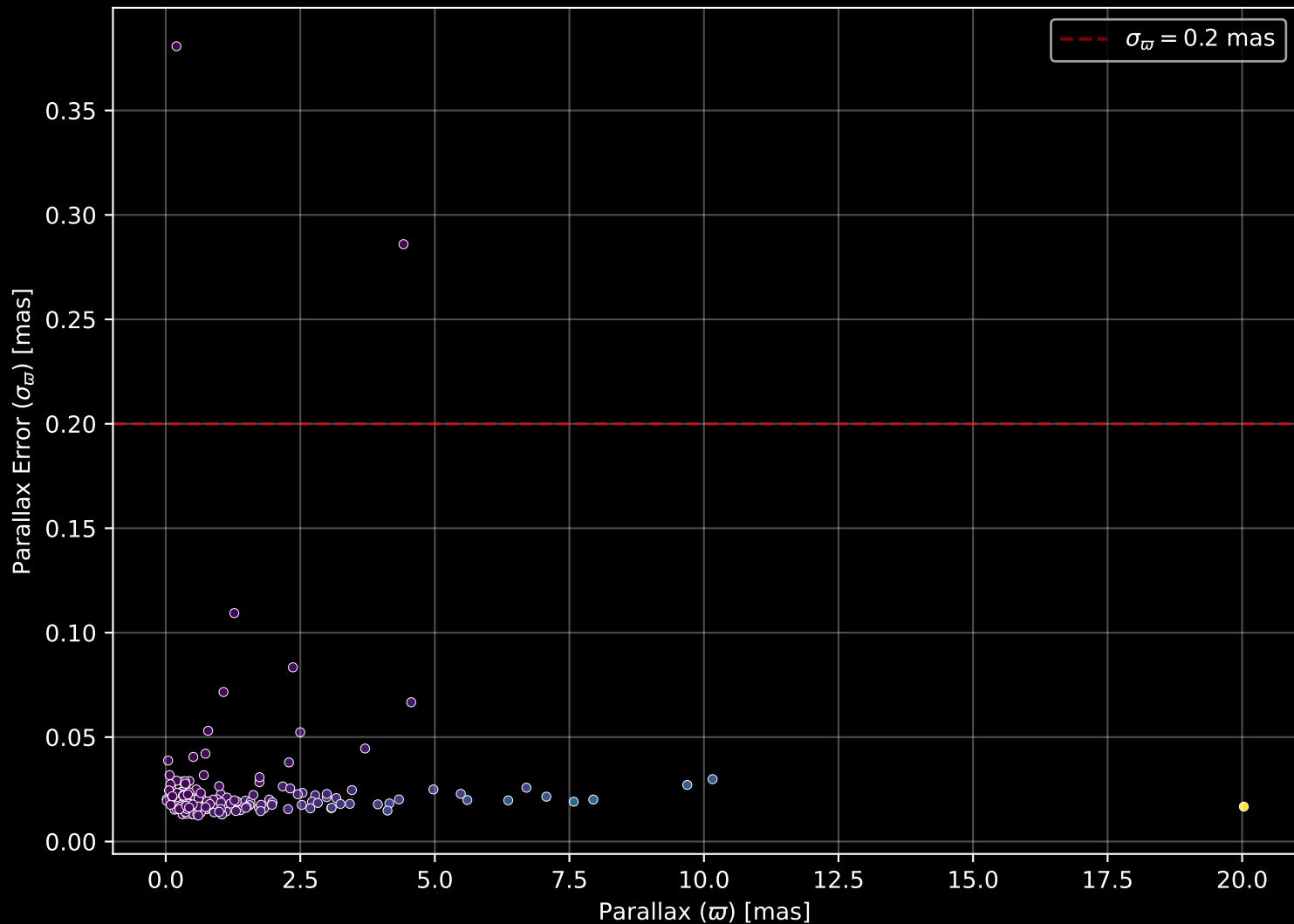
APOGEE DR17 Field: [090-45] Parallax Quality (n= 174)
