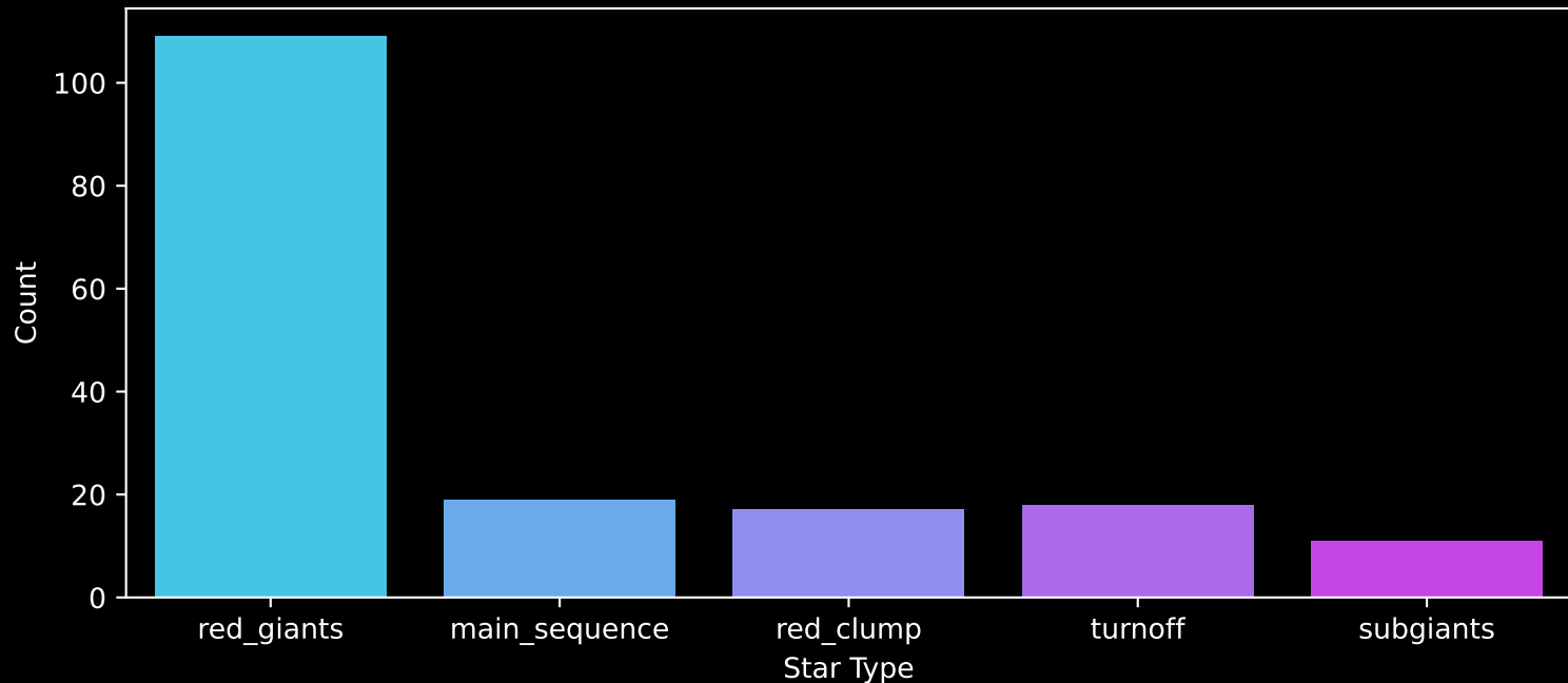
APOGEE DR17 Field: [090-45] Count plot of Star Type
