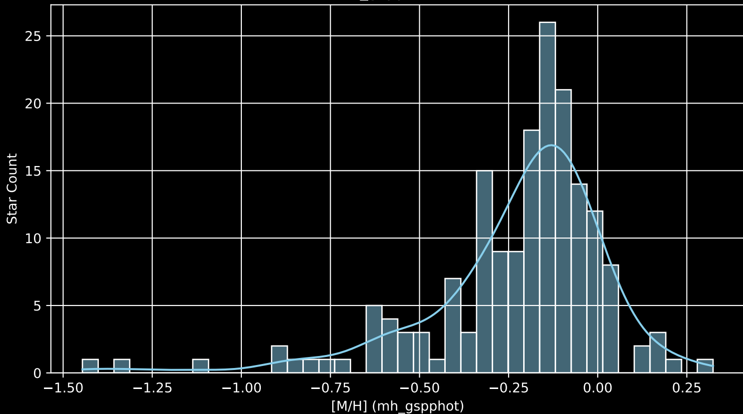
APOGEE DR17 Field: [090-45 [M/H] (mh_gspphot) (n= 174)
