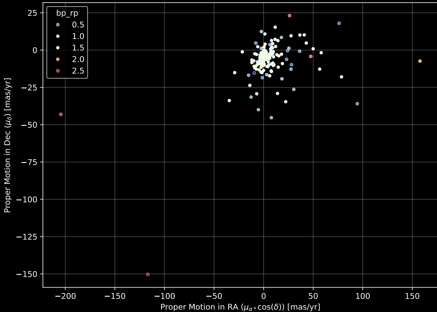
APOGEE DR17 Field: [090-45] Proper Motion Diagram (n= 174)
