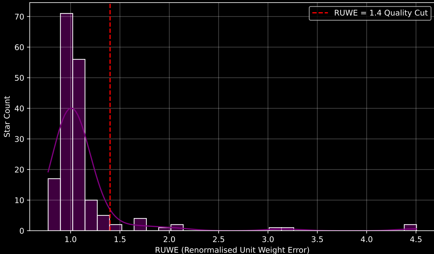
GAPOGEE DR17 Field [090-45] RUWE Distribution (n= 172)
