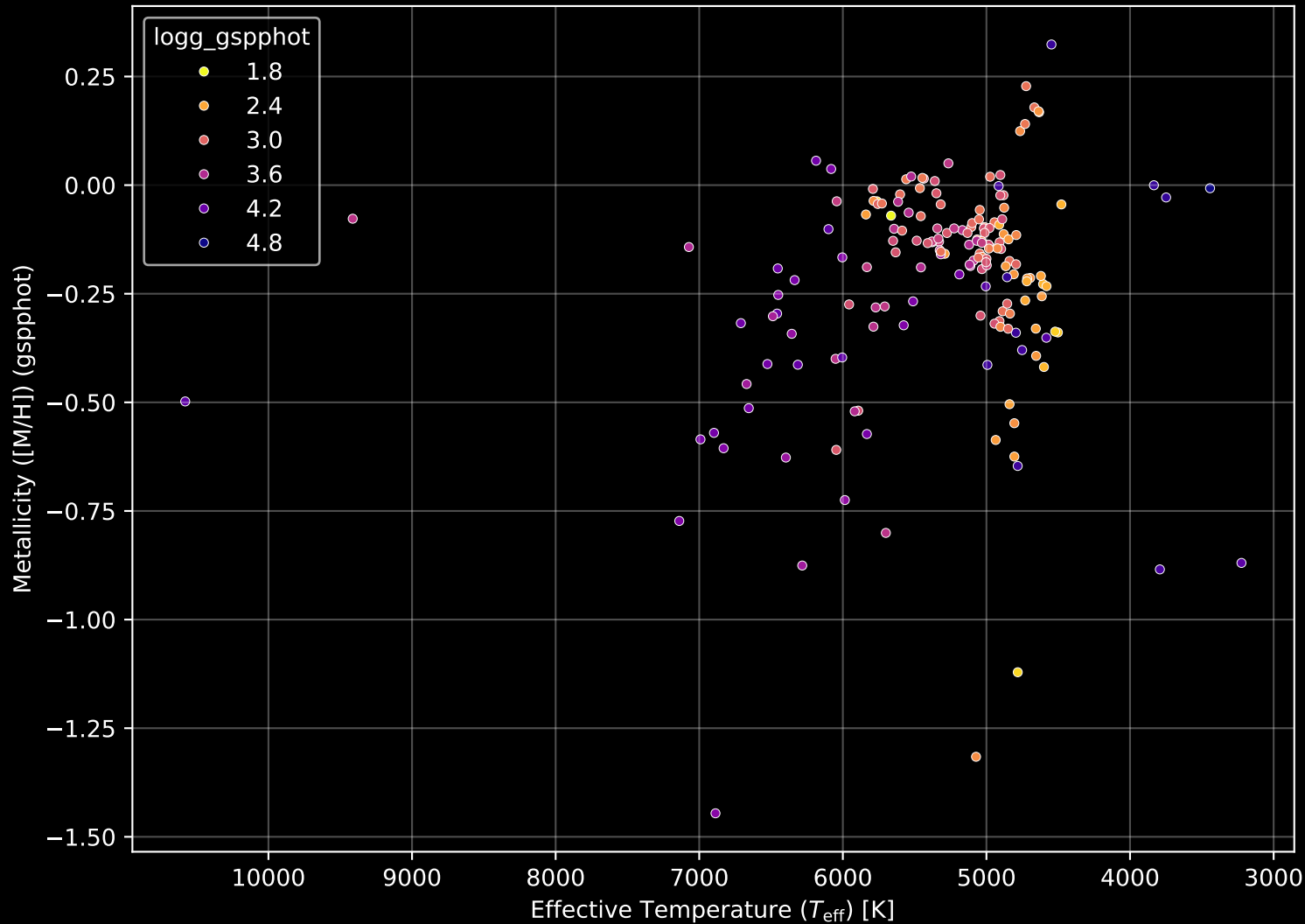
APOGEE DR17 Field: [090-45] Stellar Population Parameters (n= 174)
